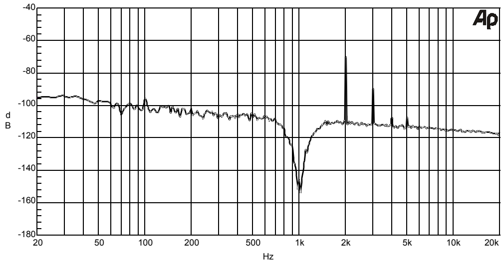
Graph 3: Distortion spectrum
